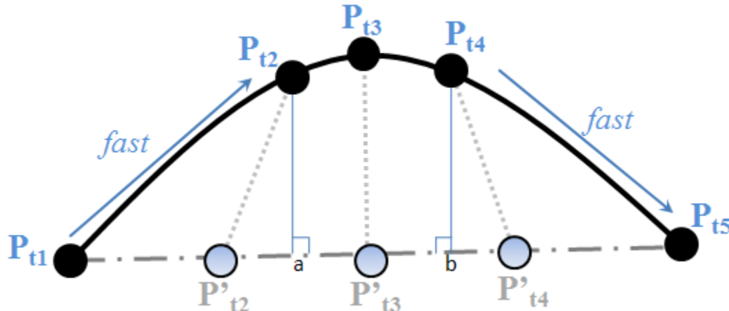
Figure 1: Synchronized Euclidean Distance measures the distance between the original and compressed trace at the same time. In contrast, line generalization algorithms ignore the temporal component and use simple perpendicular distance.
