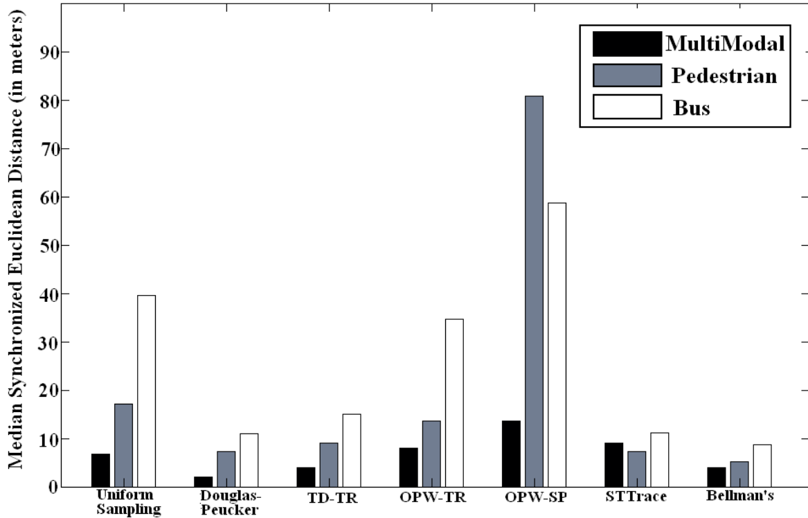
Figure 7: Difference in spatiotemporal error across different compression algorithms and travel modes. Error is measured using median synchronized Euclidean distance.
