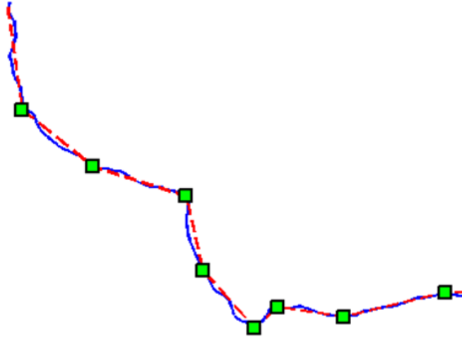
Figure 3: Douglas-Peucker Line Generalization Algorithm approximating a GPS Trajectory.
