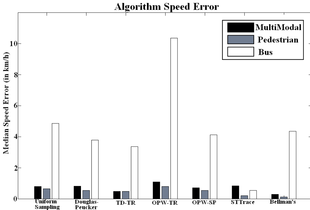
Figure 8: Difference in median speed error across different compression algorithms and travel modes.
