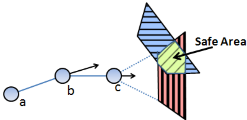
Figure 4: The STTrace Algorithm predicts the behavior of the next points based on previous GPS trajectory points. Points within the predicted Safe Area are not stored.
