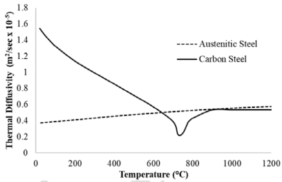
Fig. 21. Diffusivity comparison
