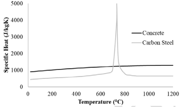
Fig. 4. Specific Heat
