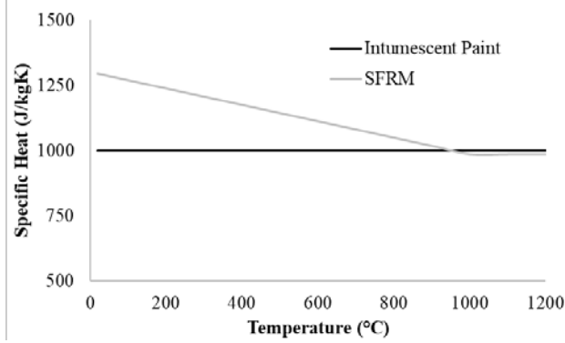
Fig. 25. Specific Heat - SFRM and IP
